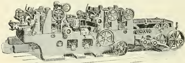
No. 17 TRIPLE-CYLINDER "LIGHTNING" FLOORER
